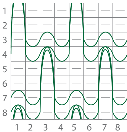
Weaving Sequence (single repeat)
