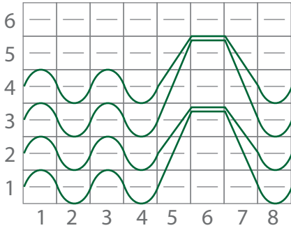
Weaving Sequence (single repeat)
